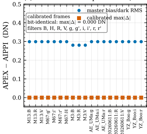
(c) APEX vs AIPPI equivalence (real data)
