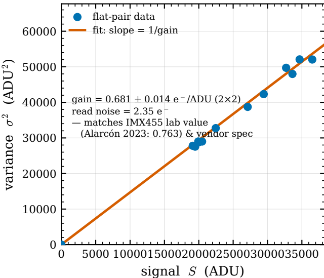
(a) Gain from the photon-transfer slope
