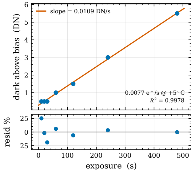
(b) Dark-current ladder
