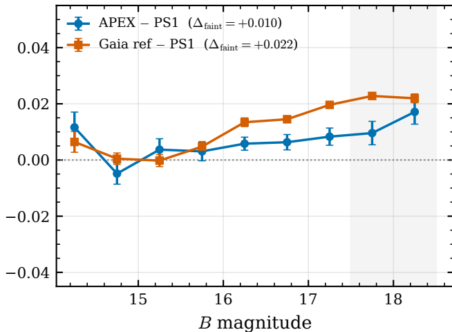
(a) B band — Gaia BP-based ref
