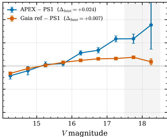
(b) V band — Gaia G-based ref
