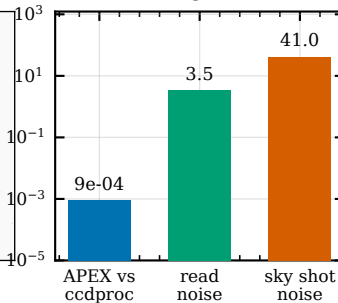
(h) noise budget (DN)
