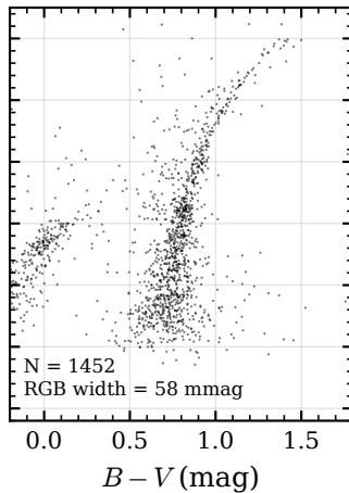
(b) PSF (step 8)
