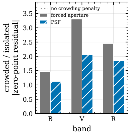
(c) crowding penalty
