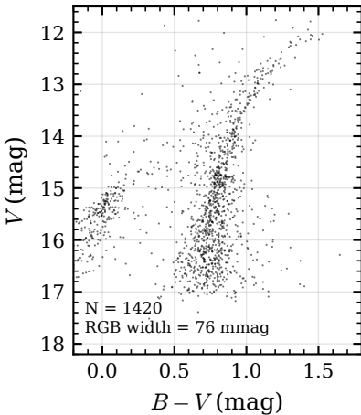
(a) forced aperture
