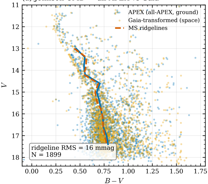
(a) Johnson CMD — all-APEX vs Gaia
