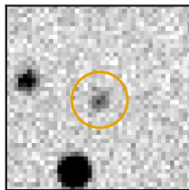
m = 17.5 ( C \approx 75\% )
