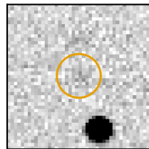
m = 18.3 ( C \approx 0\% )
