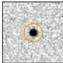
m = 16.0 ( C \approx 100\% )
