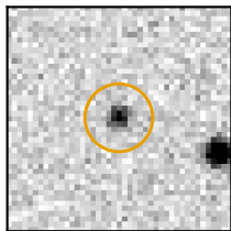
m = 17.0 ( C \approx 100\% )
