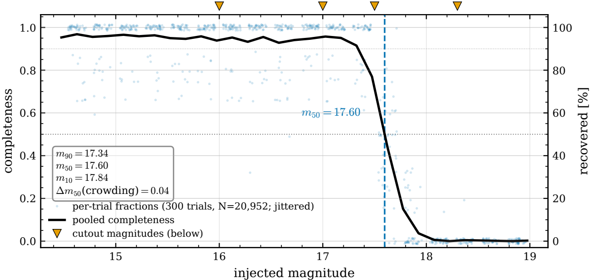
m = 16.0 ( C \approx 100\% )
