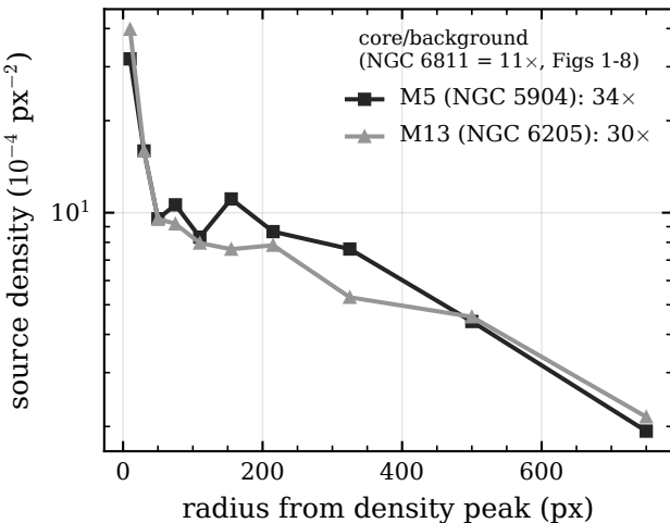
(a) globular-core density enhancement
