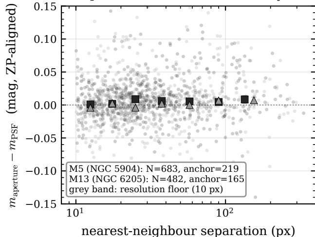
(b) aperture vs PSF vs local density
