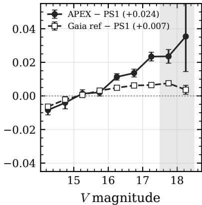
(b) V: faint-end drift
