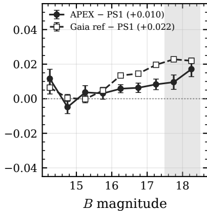
(a) B: faint-end drift
