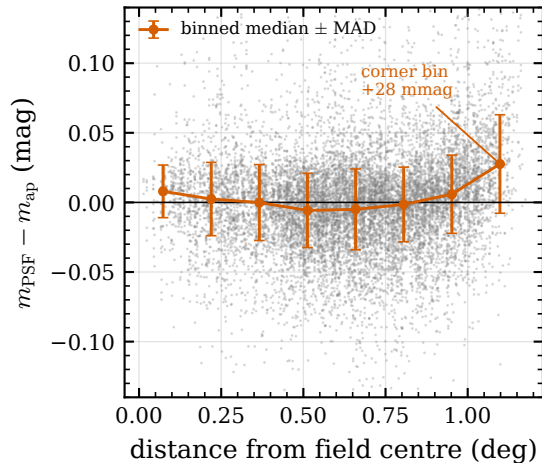
(b) M45 2.0° field, one EPSF per frame
