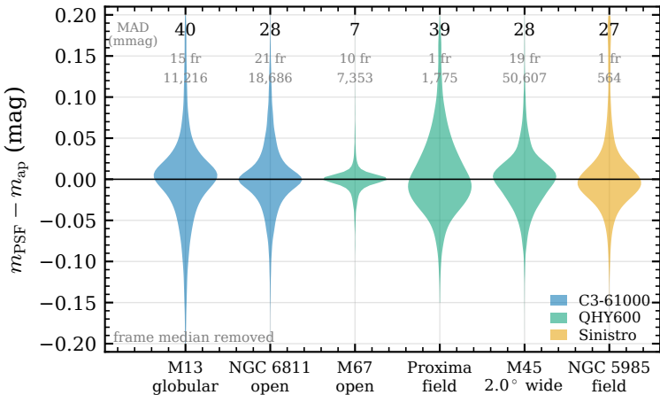
(a) star-level agreement, three cameras
