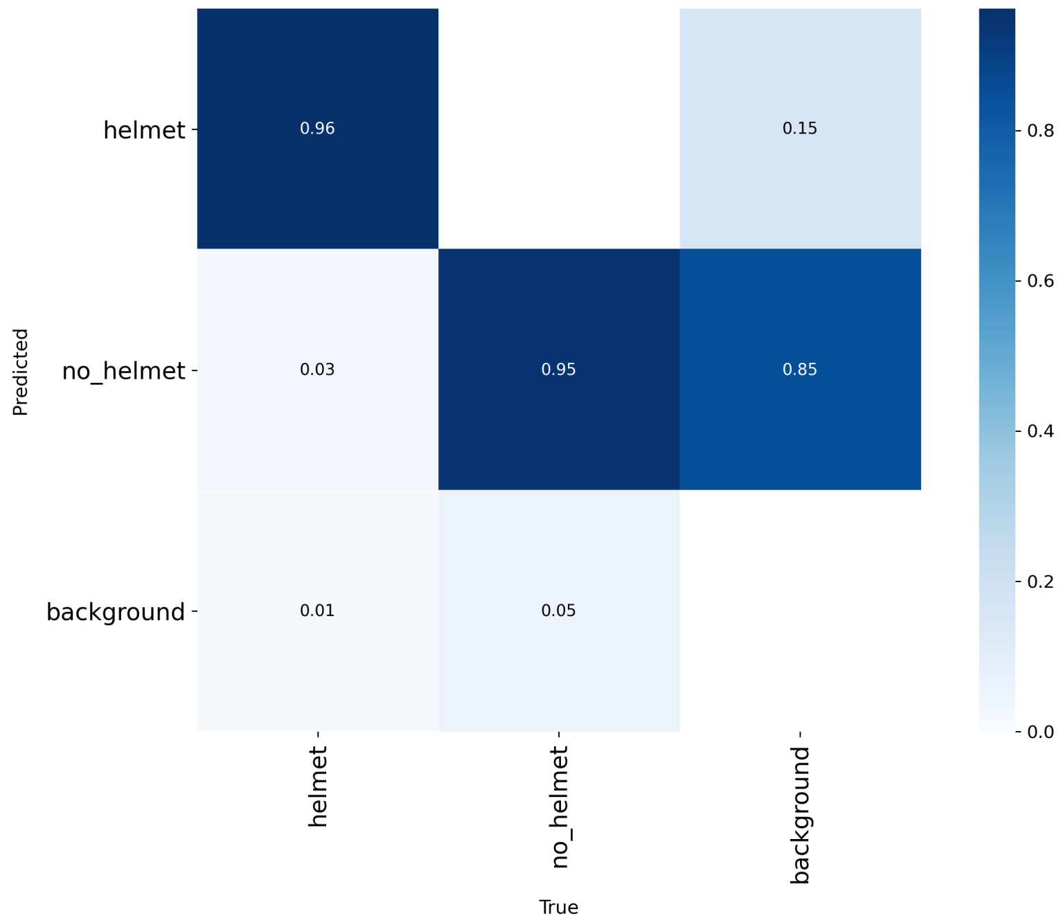
Confusion Matrix Normalized
