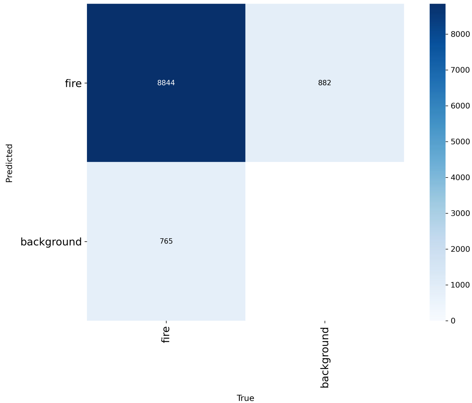
Confusion Matrix
