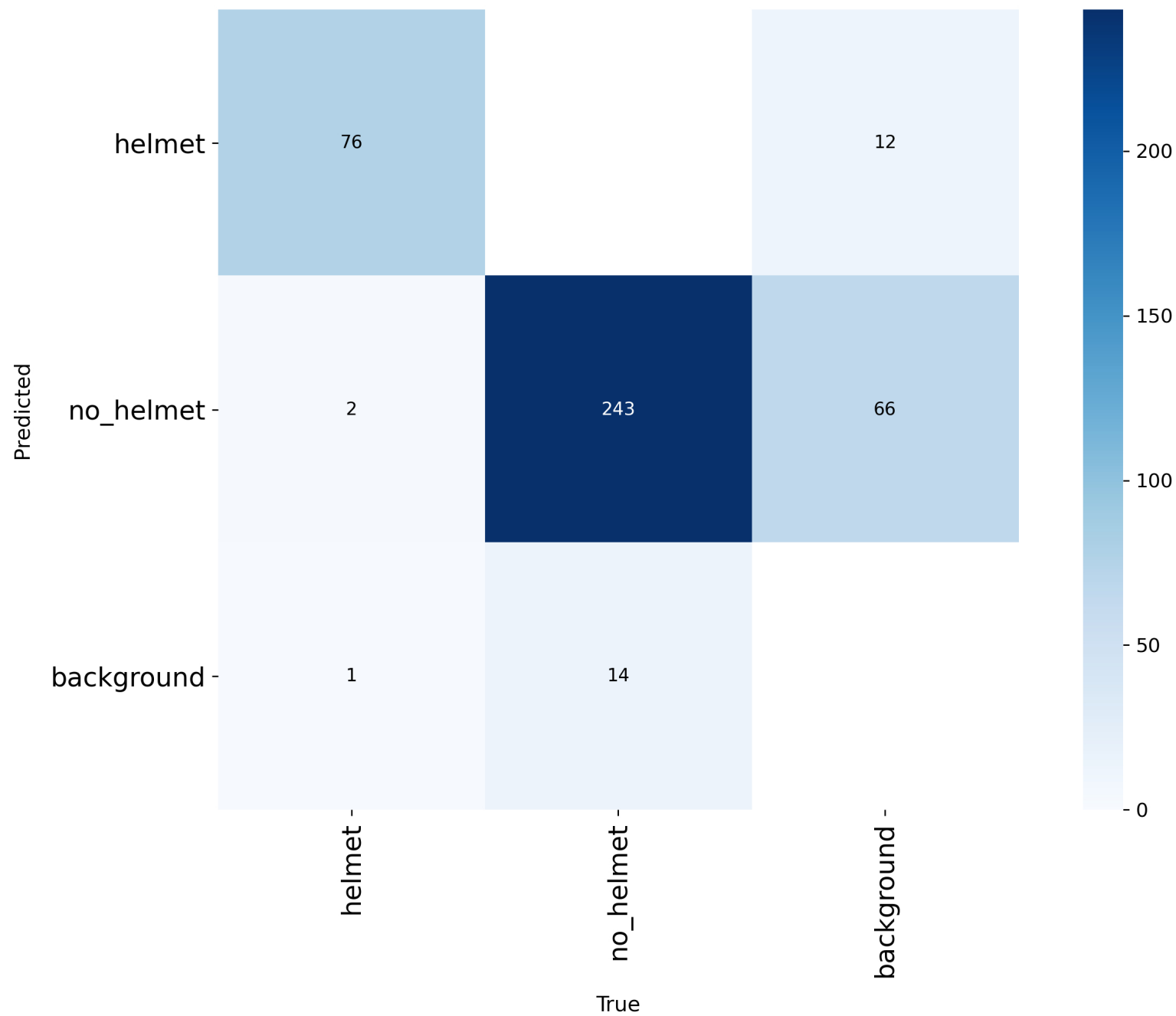
Confusion Matrix
