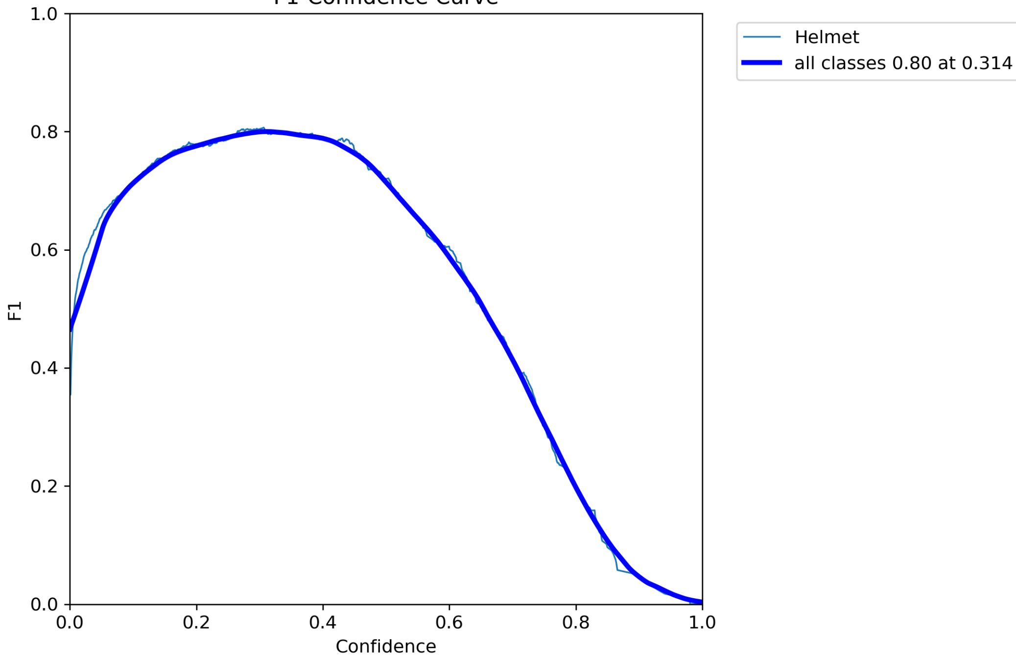
F1-Confidence Curve
