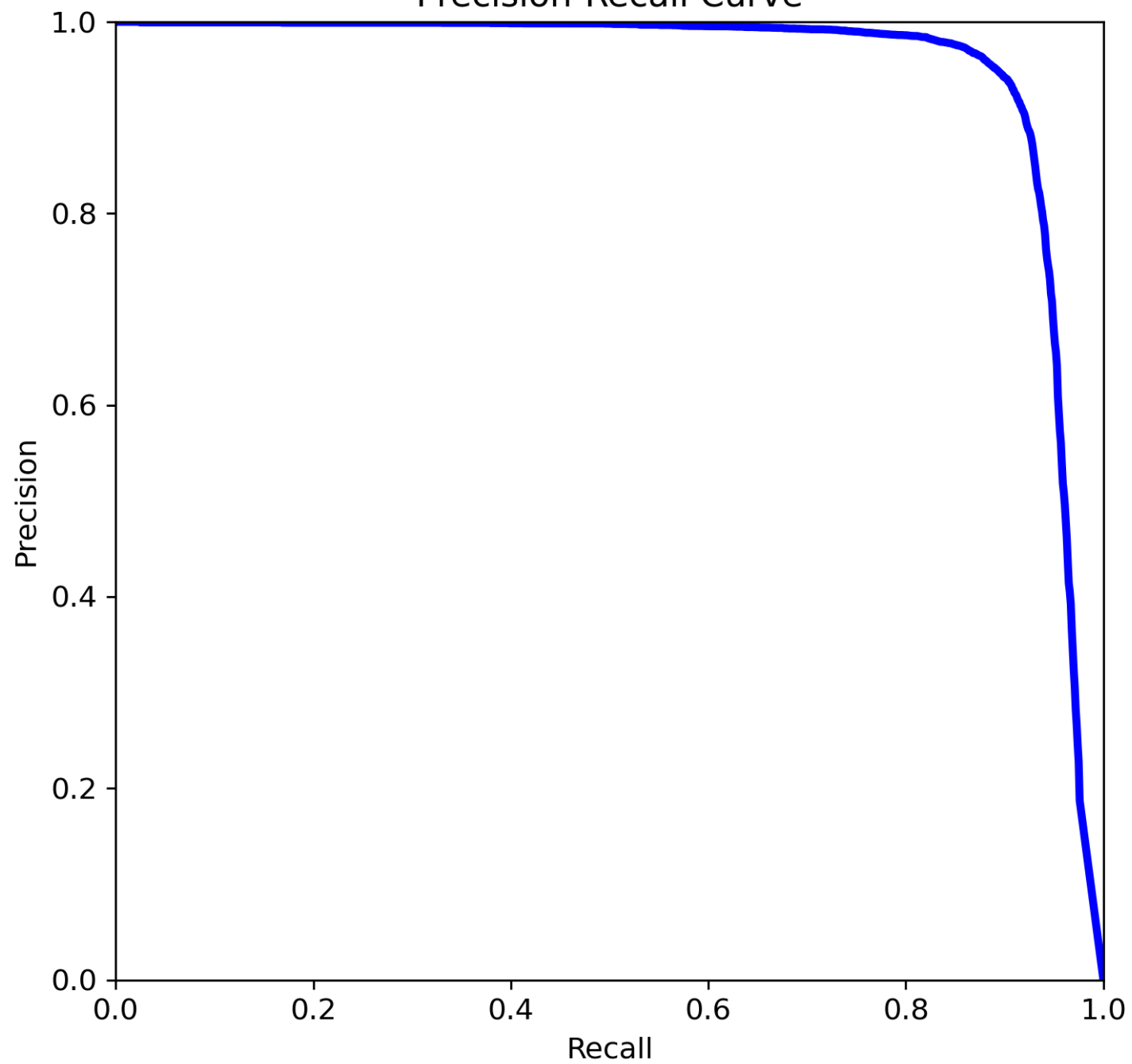
Precision-Recall Curve
