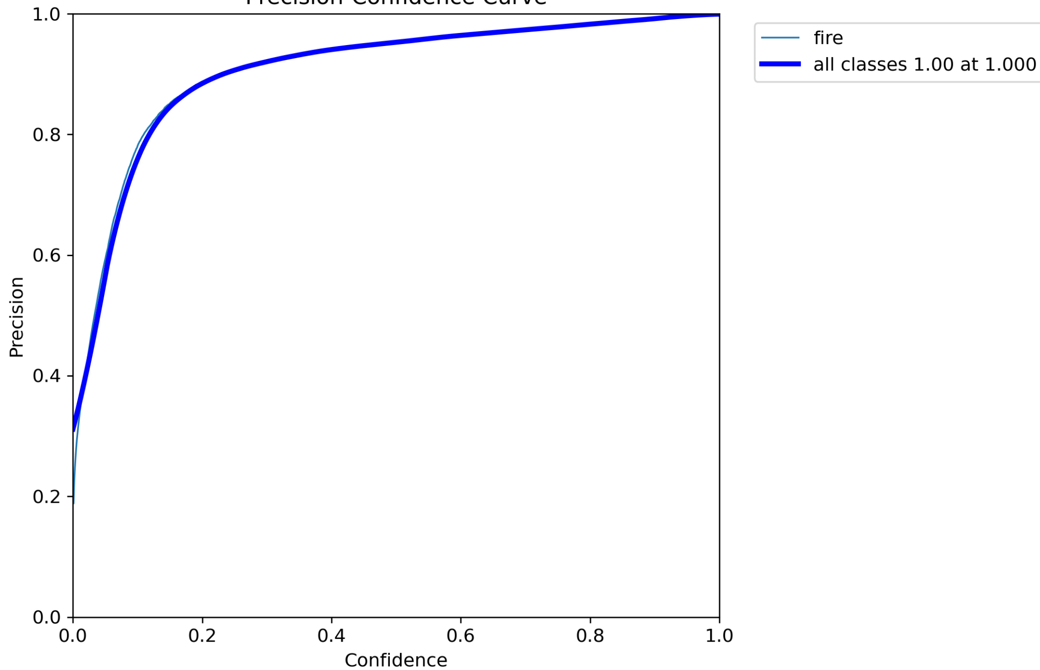
Precision-Confidence Curve
