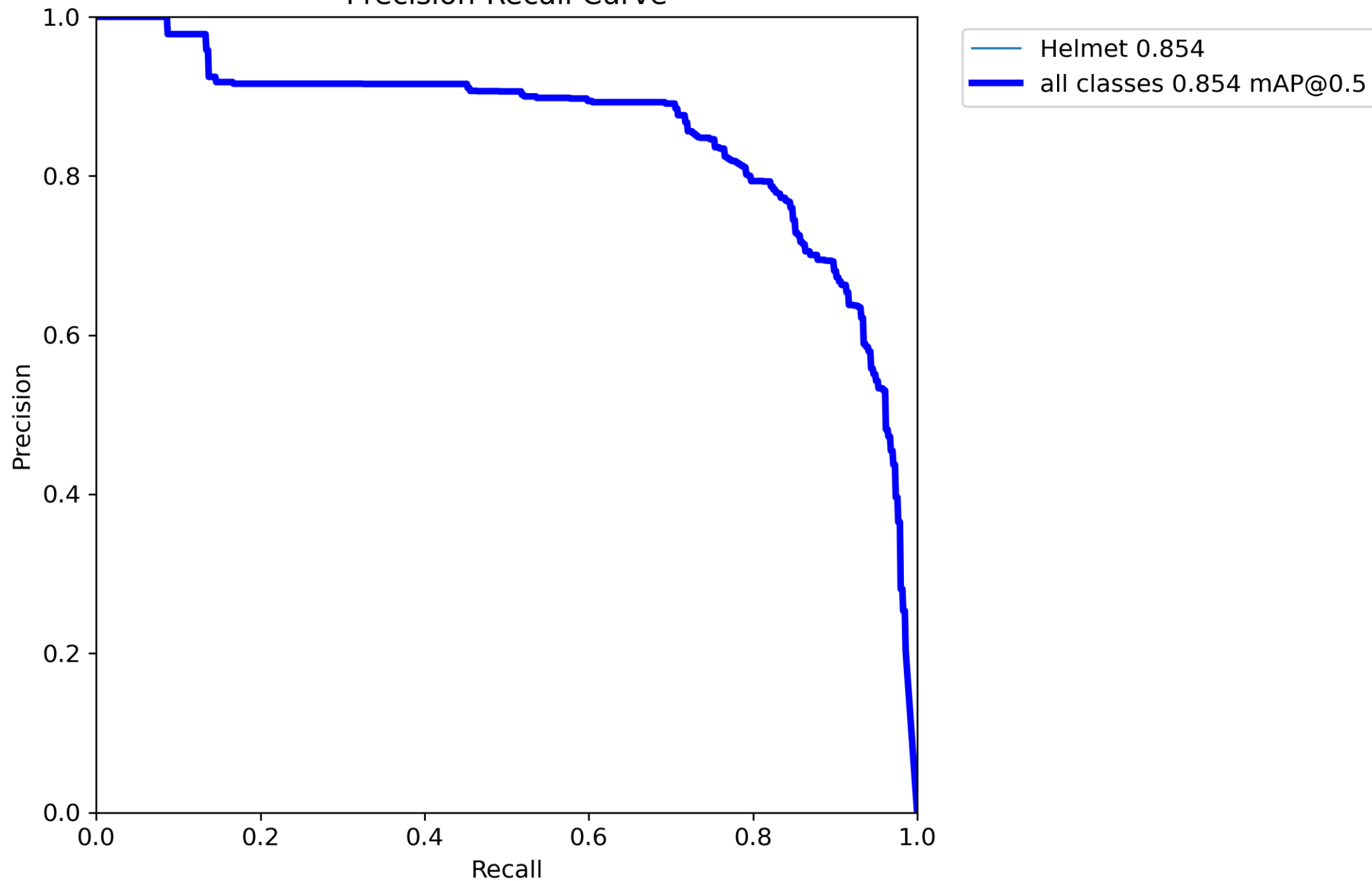
Precision-Recall Curve
