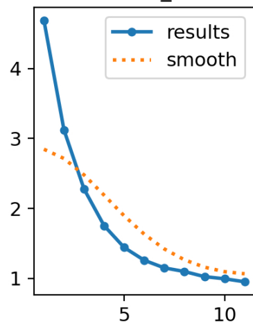
val/cls_loss
