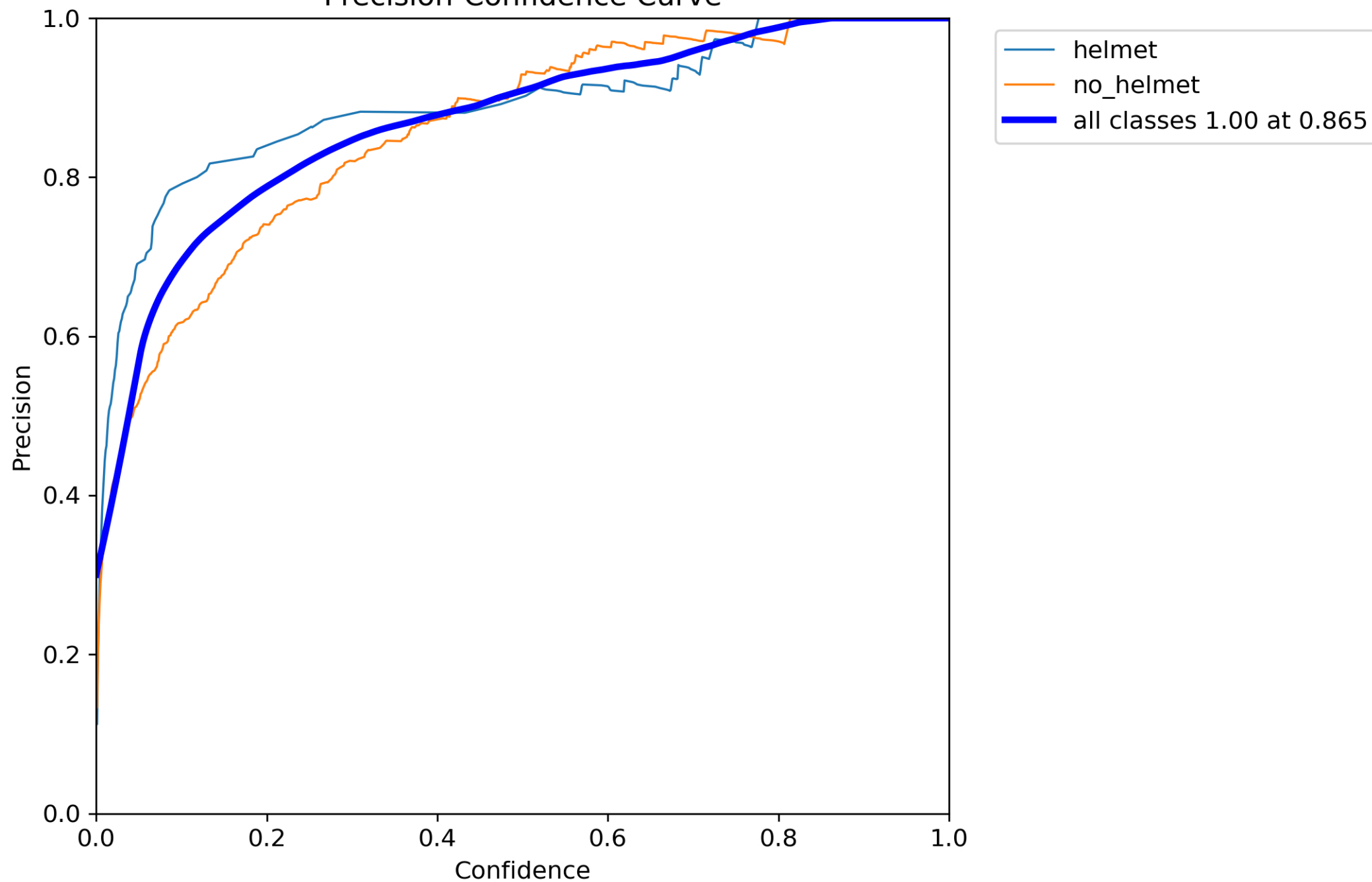
Precision-Confidence Curve
