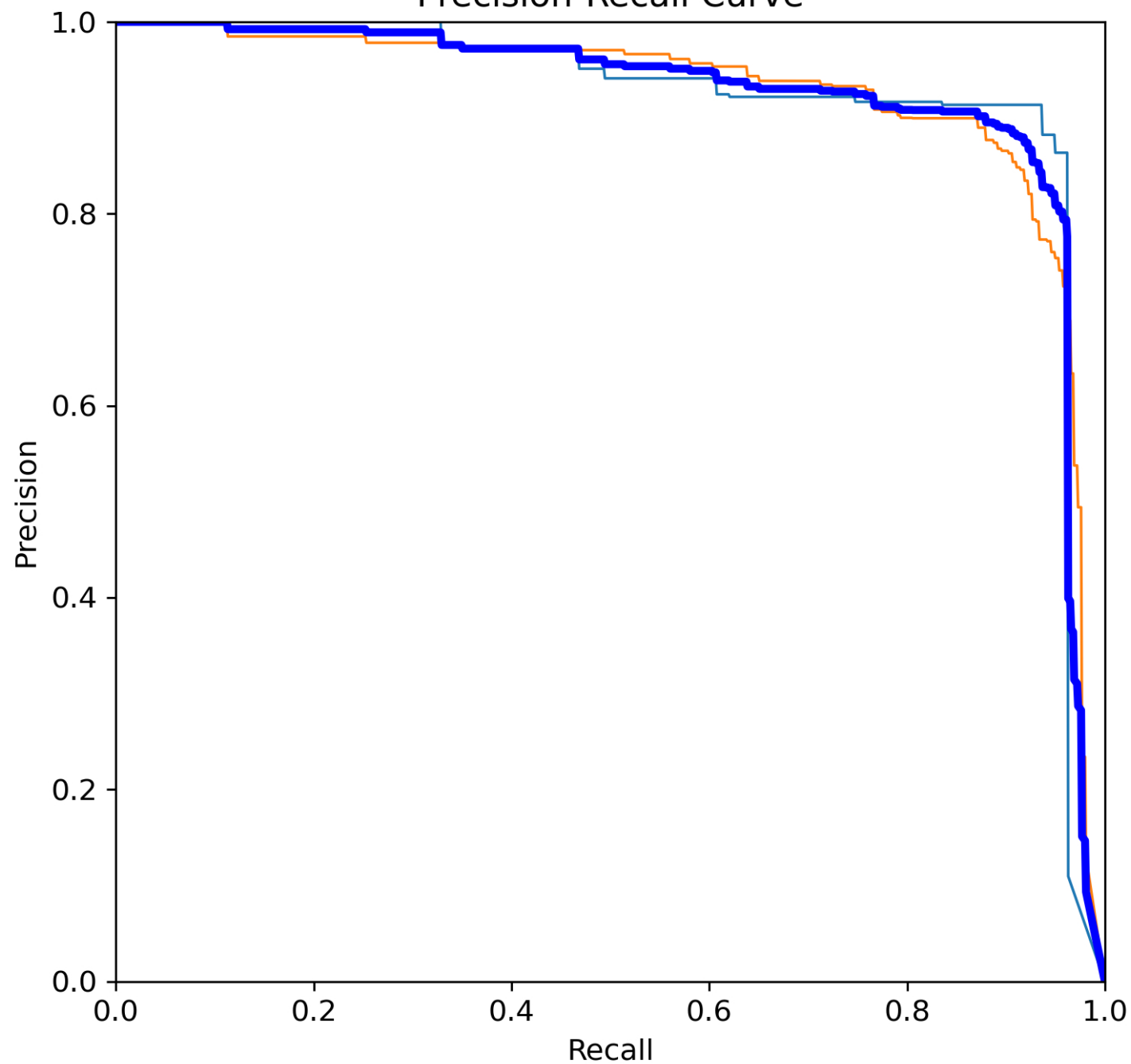
Precision-Recall Curve
