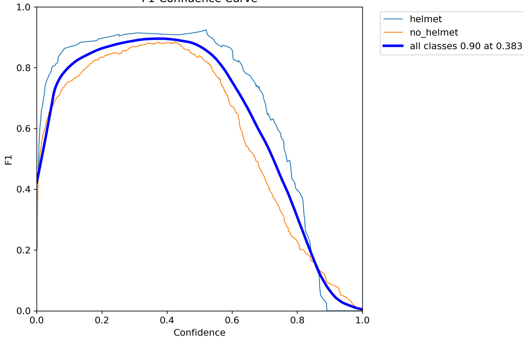
F1-Confidence Curve
