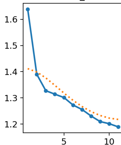
val/df_l_loss
