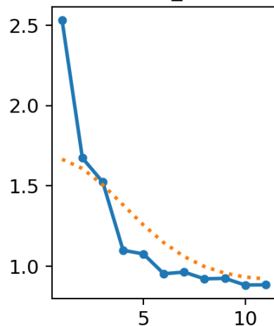
val/cls_loss
