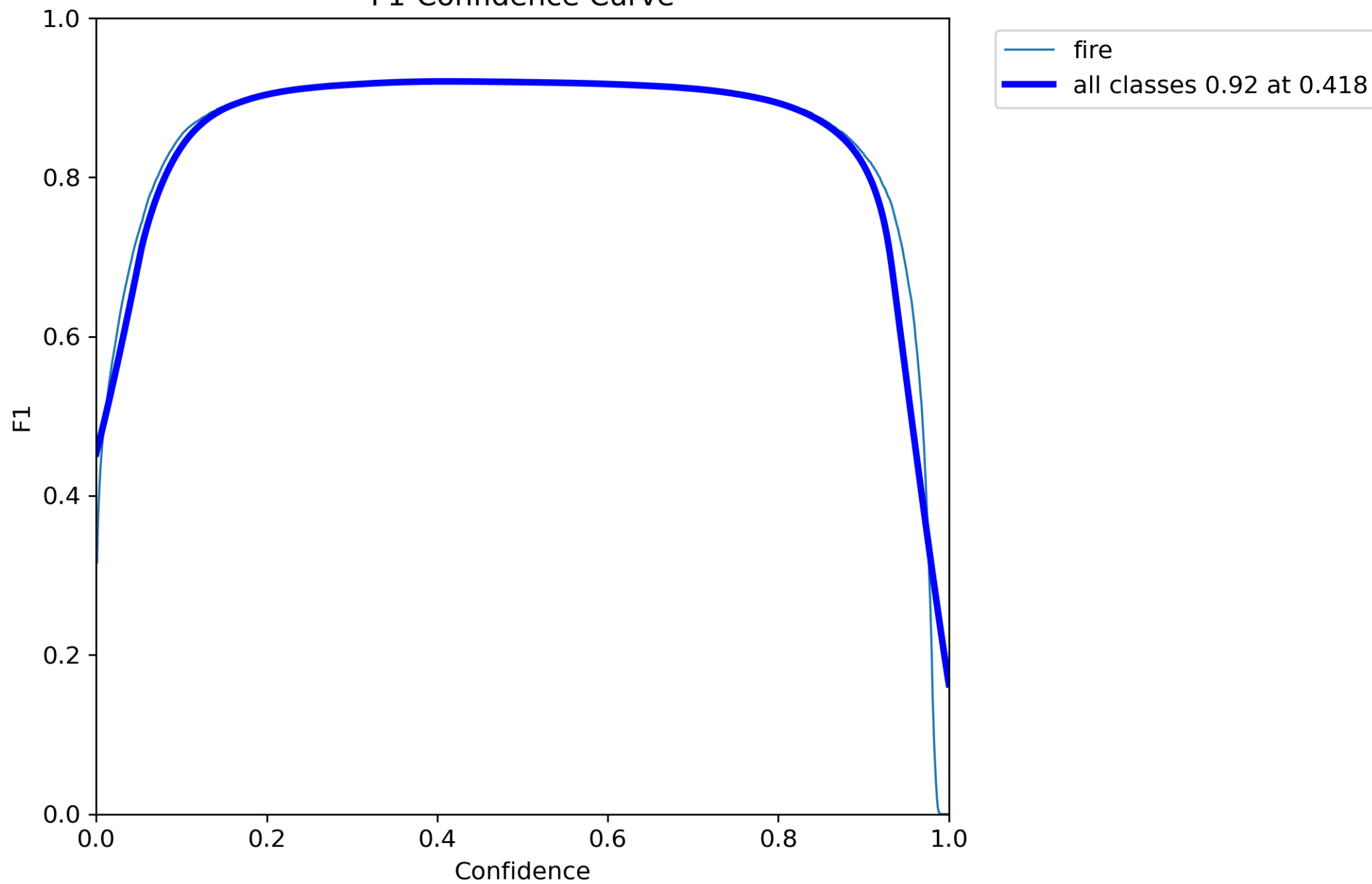
F1-Confidence Curve
