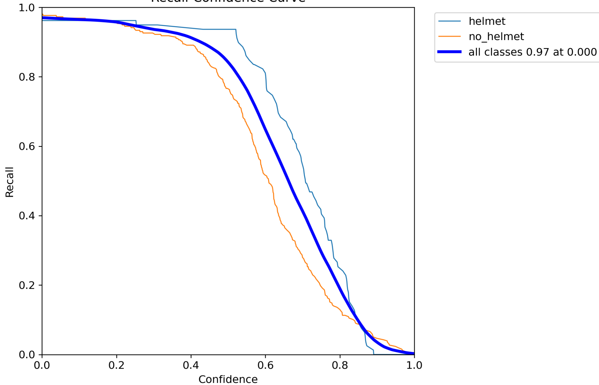
Recall-Confidence Curve
