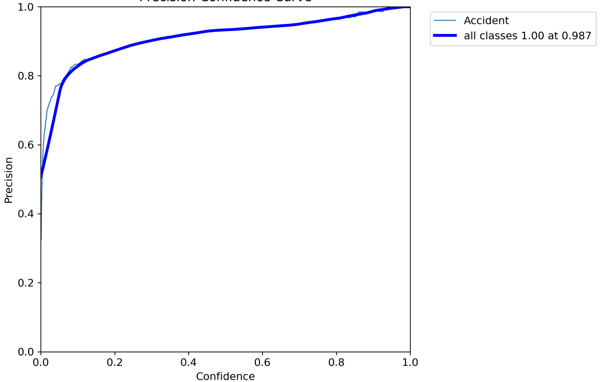
Precision-Confidence Curve
