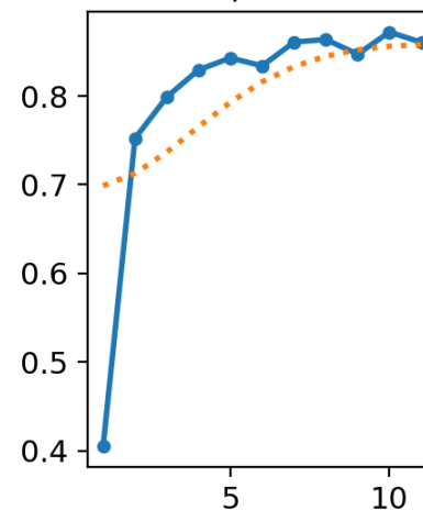
metrics/mAP50(B)
