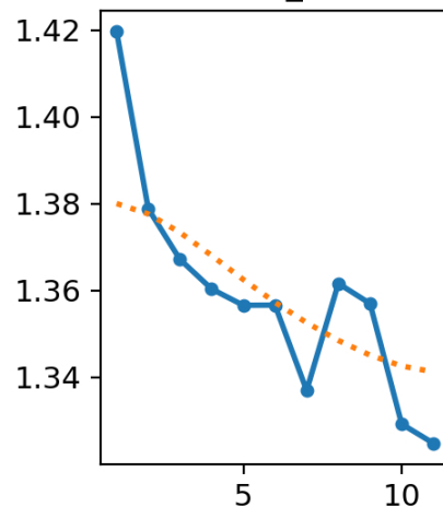
val/df_l_loss
