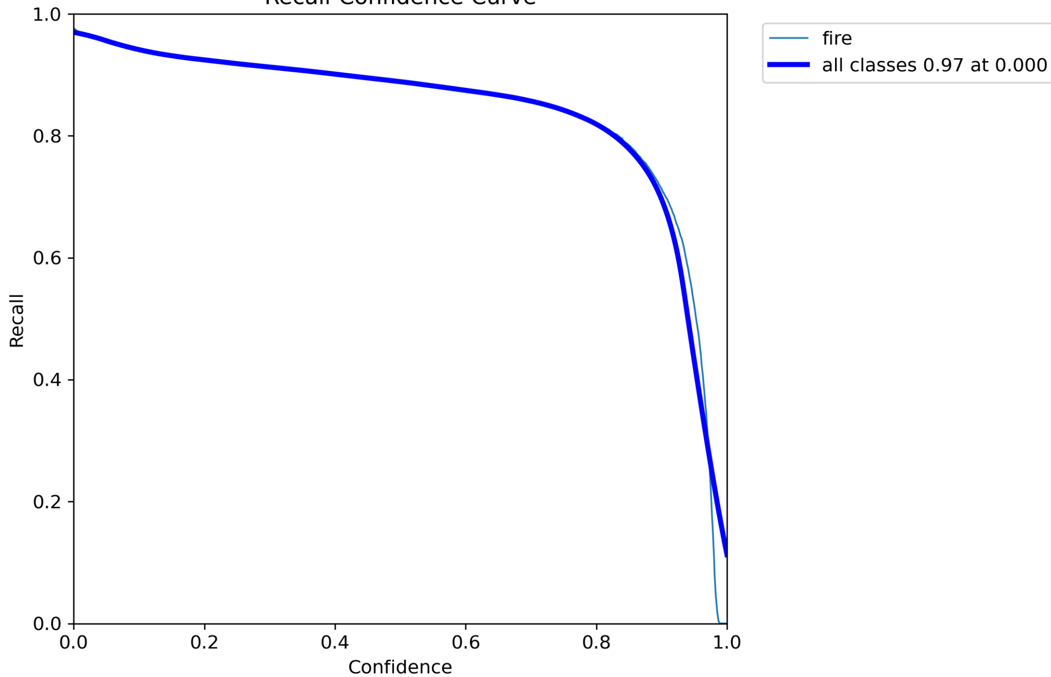
Recall-Confidence Curve
