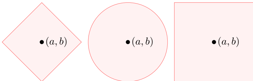
(a) d_1 -ball centred at (a, b) (b) d_2 -ball centred at (a, b) (c) d_\infty -ball centred at (a, b)
