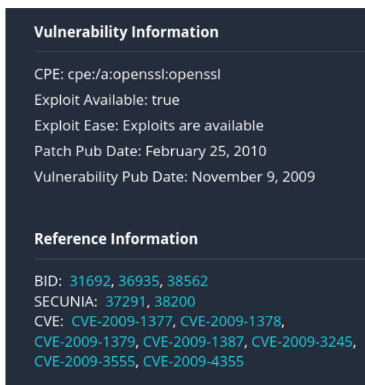
FIGURE A5: CVE id information from FIGURE A4. Find CVE id that can be attacked using Metasploit by referring to exploit-db.com or nvd.nist.gov .
