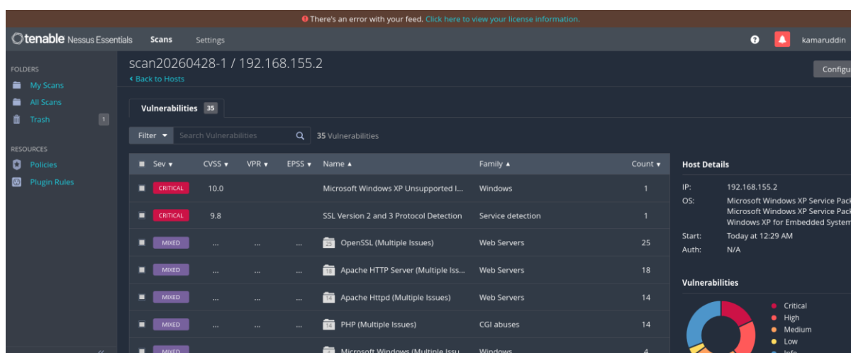
FIGURE A3: Details of vulnerabilities. Look for vulnerabilities with higher CVSS ranking values. CVSS values are between 0-10. CVSS value of 10 is the most CRITICAL, and most vulnerable for attack.
