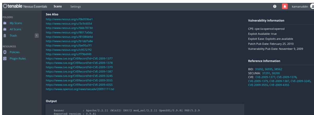
FIGURE A5: Show details of chosen vulnerability with CVE id information.
