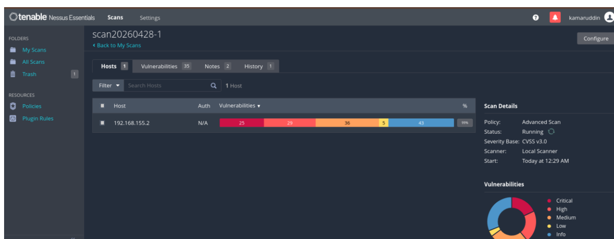
FIGURE A2: This is the result of the scan. Click on the Vulnerabilities (e.g. on the RED box@CRITICAL) to view details.
