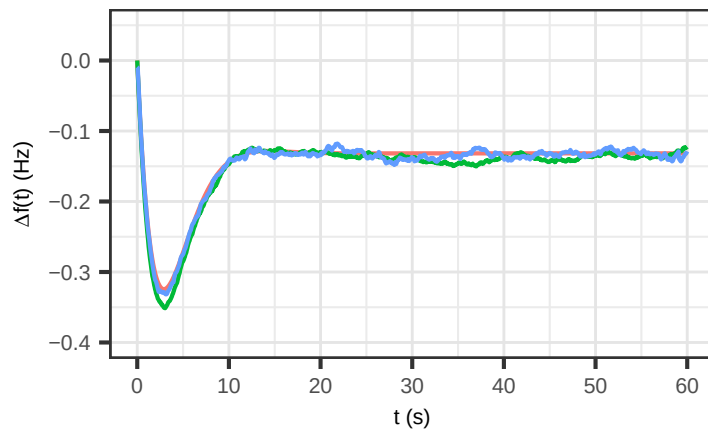
Frequency Derivatives from converter_not_big_noise.
