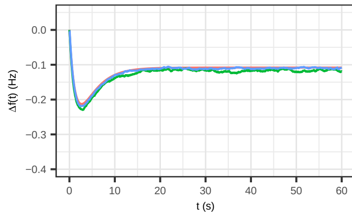
Frequency Derivatives from converter_yes_big_noise.
