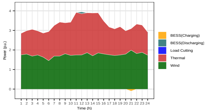
Fig. 5. Power balance process of the IEEE 6-bus system with DCCs.
