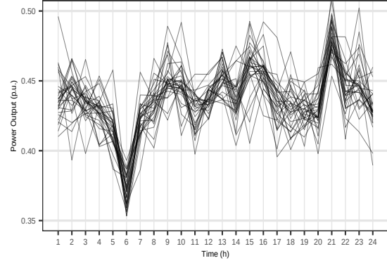
Fig. 3. Chronological stochastic output generated by wind farms.
