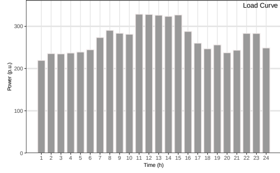
Fig. 2. Chronological load curve of the IEEE 6-bus system with DCCs.
