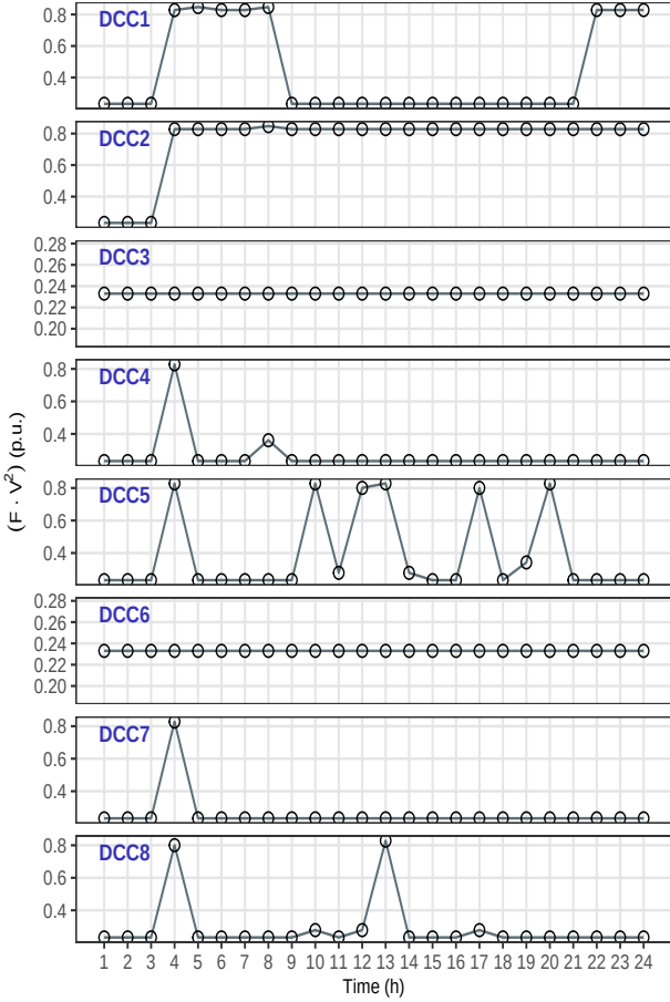
Fig. 7. sequential frequency regulations through DVFS in DCCs.
