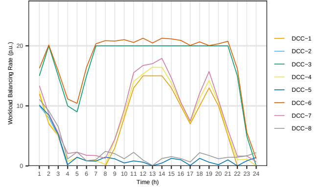
Fig. 4. Given workload distribution of the IEEE 6-bus system with DCCs.
