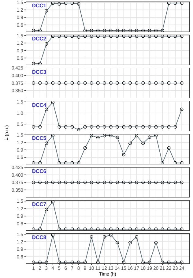
Fig. 8. sequential workload balancing through DVFS in DCCs.
