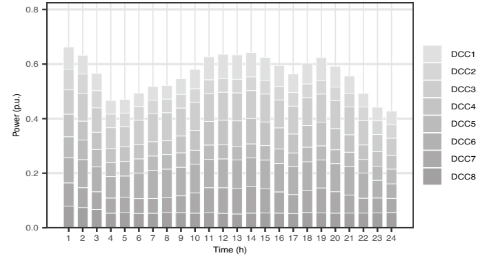
Fig. 9. Sequential workload consumption generated by multiple DCCs reallocation (intervals = 4h).
