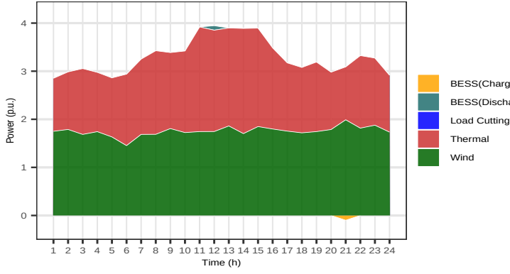
Fig. 7. Power balance process of the IEEE 6-bus system considering workload consumptions hosted by DCCs.
