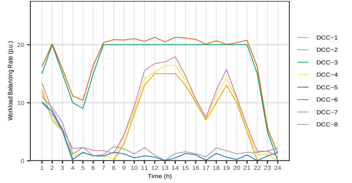
Fig. 4. Workload distribution of multiple DCCs.
