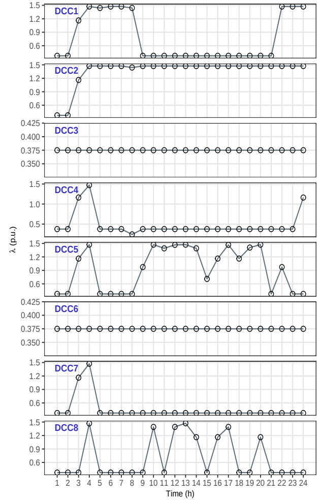
Fig. 7. sequential workload balancing through DVFS in DCCs.
