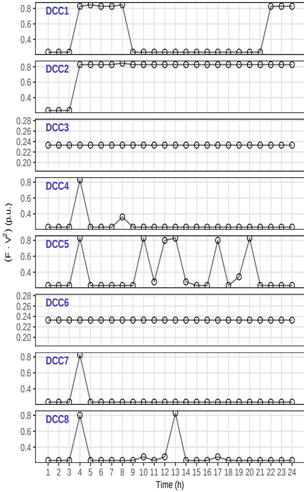
Fig. 8. sequential frequency regulations through DVFS in DCCs.
