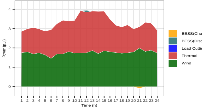
Fig. 5. Power balance process of the IEEE 6-bus system with DCCs.
