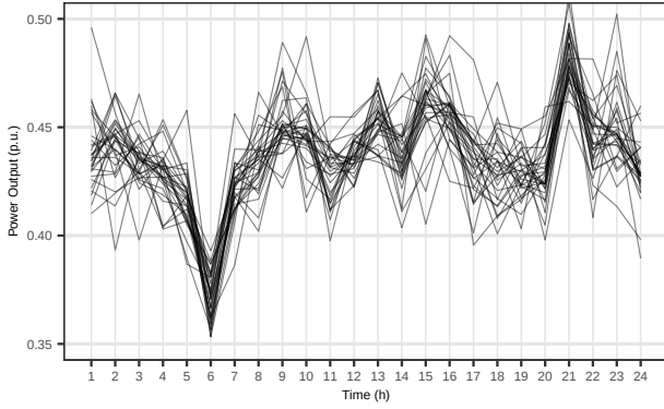
Fig. 3. Chronological stochastic output generated by wind farms.
