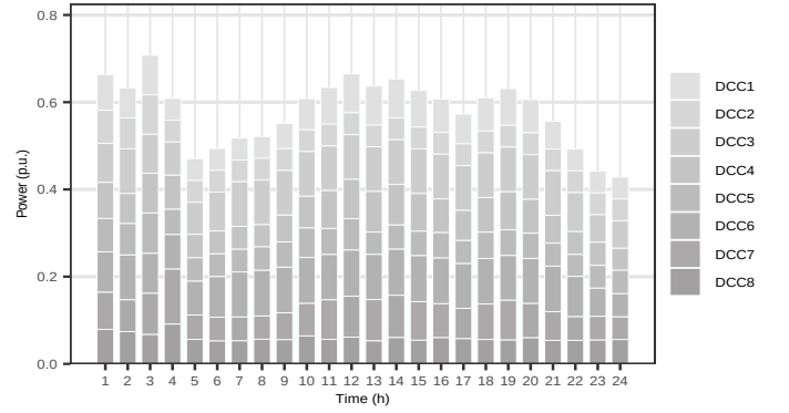
Fig. 6. sequential workload consumption generated by DCCs.
