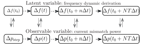
Figure 1. The time-discretized status recurrence process of frequency derivation in the proposed BF-SFR method
