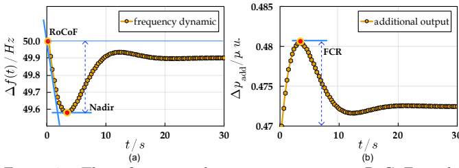
Figure 2. Three frequency dynamic requirements: RoCoF , nadir and FCR
