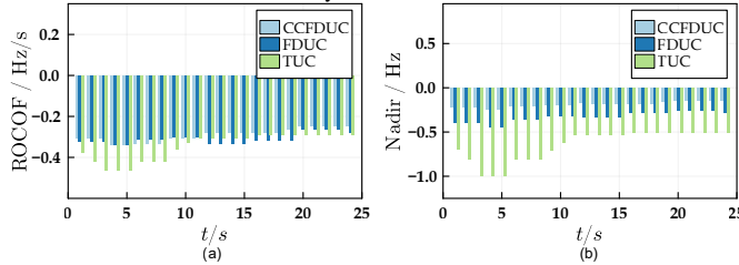
Figure 13. The distribution of RoCoF in (a) and nadir in (b) corresponding to scheduled commitments through TUC/FDUC/CCFDUC in the modified IEEE 118 bus test system.
