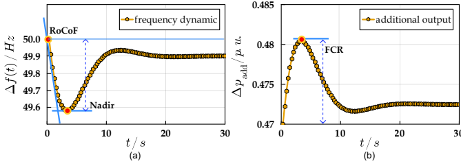
Figure 2. Three frequency dynamic requirements: RoCoF , nadir and FCR serving as reserves during imbalanced disturbances, [5, 11]. In combination with (3), the binding of the additional power \langle \Delta p_{add}^G, \Delta p_{add}^W, \Delta p_{add}^E \rangle from different units is obtained, i.e., \sum_{g=1}^{NG} p_{g,s,t} \geq \Delta p_{add}^G(t) ; \sum_{w=1}^{NG} p_{w,s,t} \geq \Delta p_{add}^W(t) and \sum_{e=1}^{NE} p_{e,s,t} \geq \Delta p_{add}^E(t), \forall t, s . By replacing \langle \Delta p_{add}^G(t), \Delta p_{add}^W(t), \Delta p_{add}^E(t) \rangle with their analytical formulations in ??????, another equivalent constraint regarding FCR can be derived,
