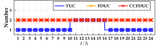
Figure 7. Cumulative numbers of activated conventional generators through TUC/FDUC/CCFDUC in the modified IEEE 6 bus test system.
