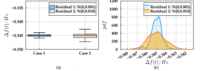
Figure 5. Statistical 1/2 and 1/4 quantile level in (a) and posterior probabilistic density distribution in (b) of \Delta f(t) at time-to-nadir under different residual conditions.
