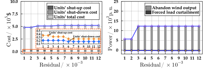
Figure 11. Change of scheduled cost and abandoned power through CCFDUC with different residual settings.
