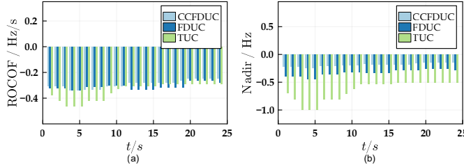
Figure 13. The distribution of RoCoF in (a) and nadir in (b) corresponding to scheduled commitments through TUC/FDUC/CCFDUC in the modified IEEE 118 bus test system.
