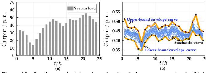
Figure 12. Load curve in (a) and stochastic wind power scenarios in (b) in the modified IEEE 118 bus test system.
