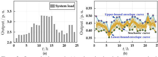
Figure 3. System load curve in (a) and stochastic wind power scenarios in (b) in the modified IEEE 6 bus test system.
