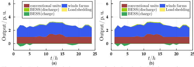
Figure 8. Active power balance curves of calculated scheduled commitments produced by TUC/FDUC/CCFDUC in the modified IEEE 6 bus test system.
