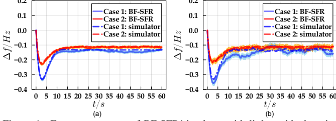
Figure 4. Frequency curves of BF-SFR/simulator with little residual setting in (a) and large residual condition in (b).
