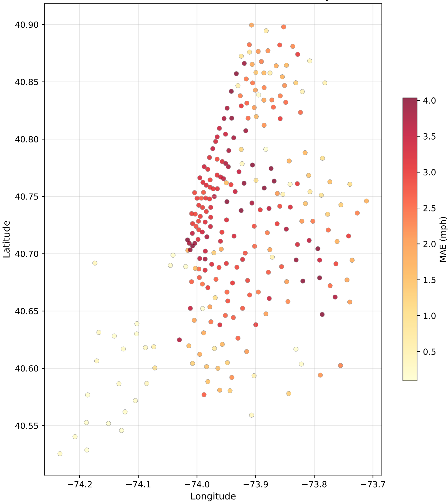
CityFlow-GNN: Per-Zone Prediction MAE (NYC Taxi Zones — centroid bubble map)
