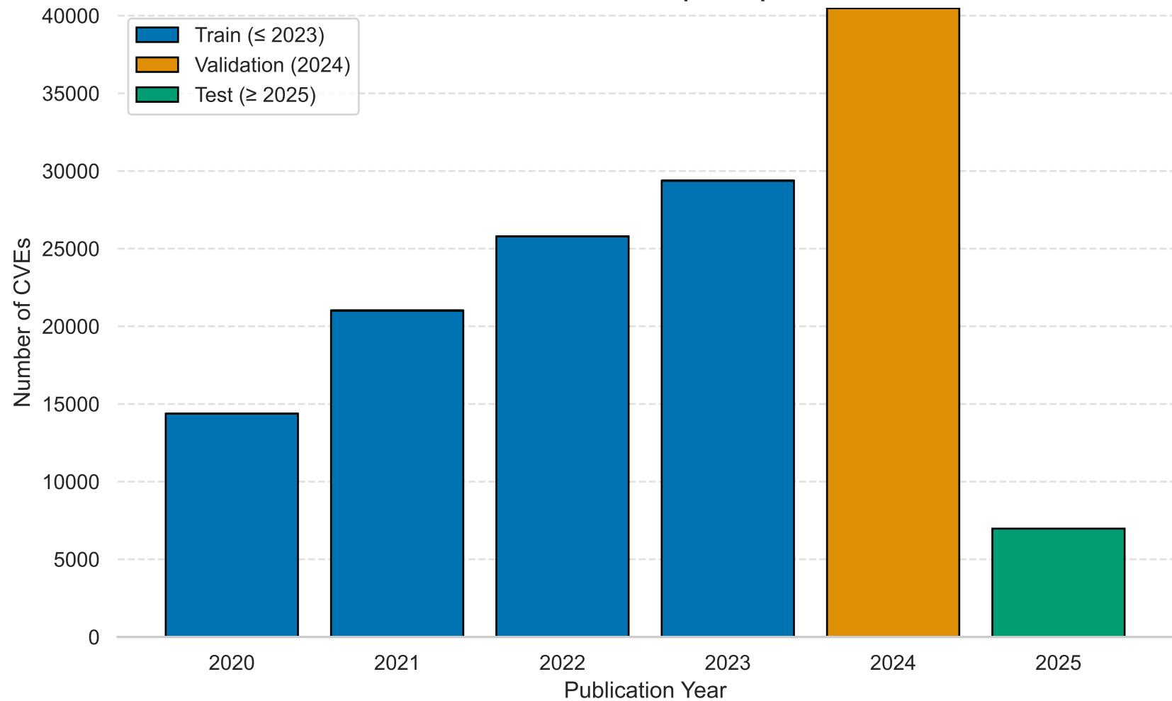
CVE Dataset Temporal Split
