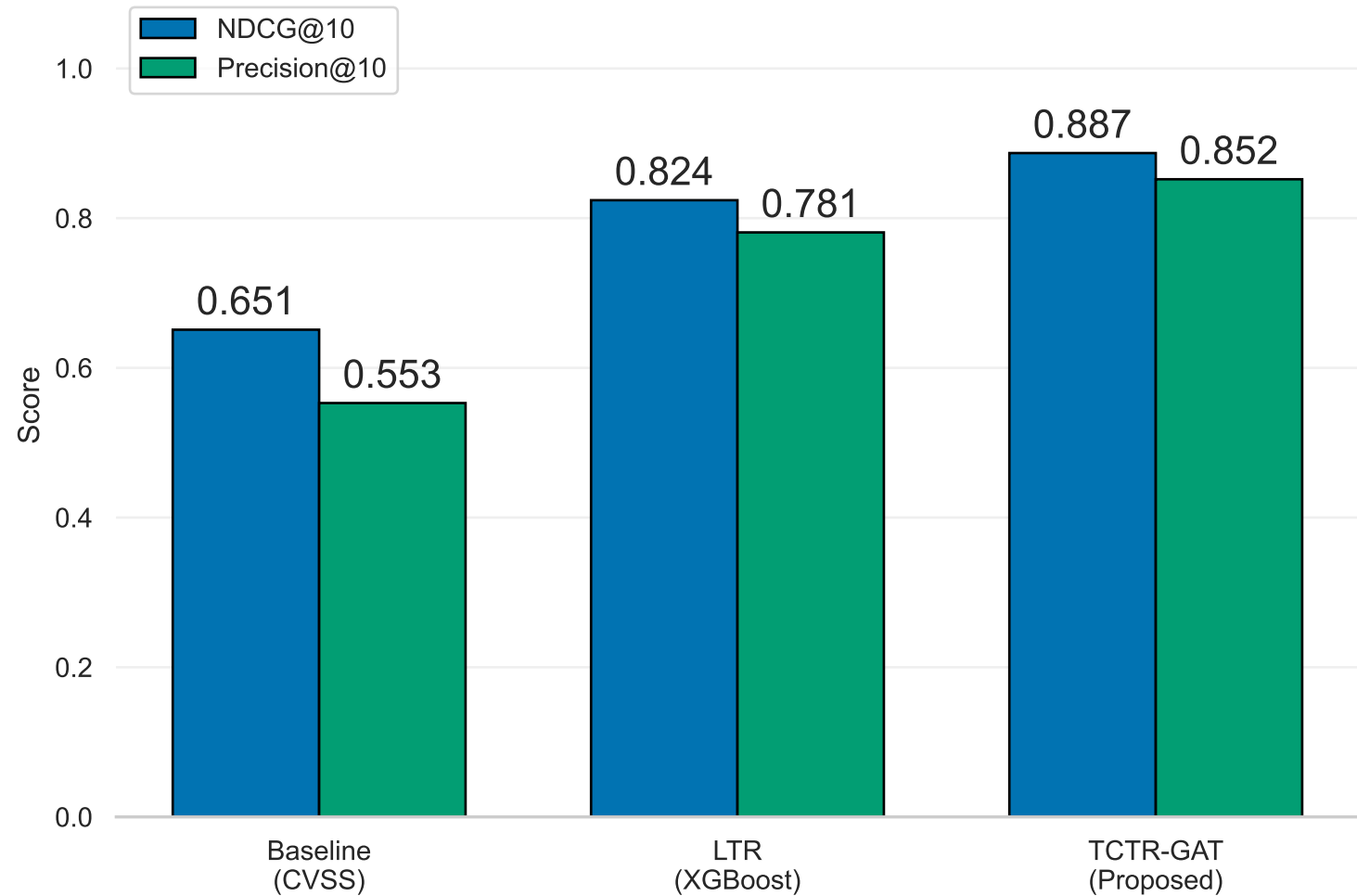
TCTR Model Performance vs Baselines
