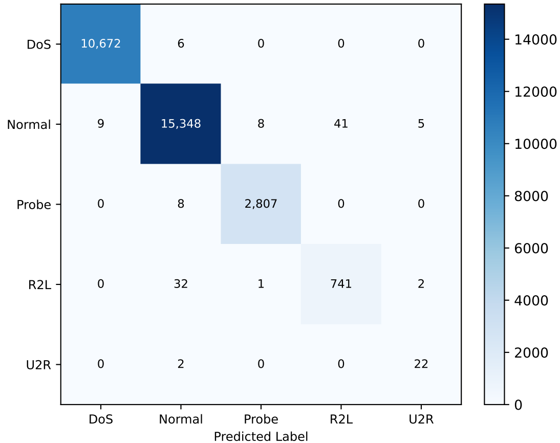
Confusion Matrix — Counts Accuracy: 99.62%
