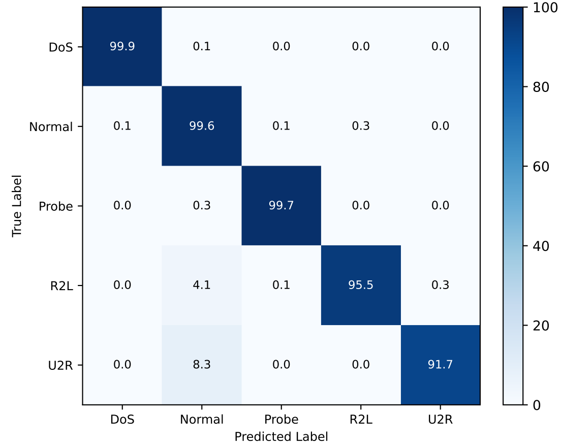
Confusion Matrix — Percentages
