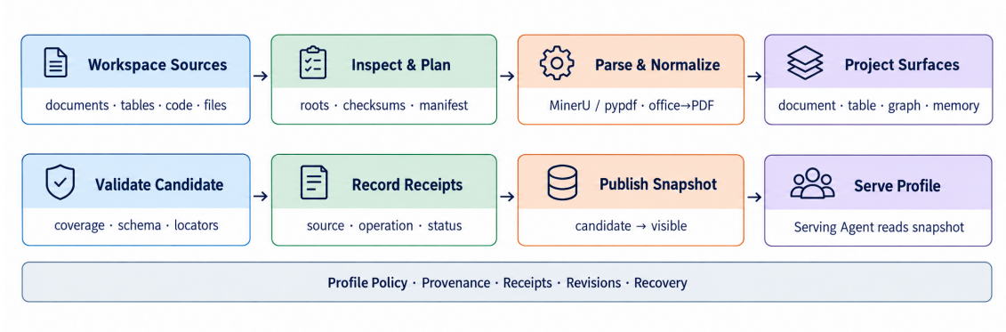
Figure 2: DataMind-Build ingestion path. The Build Agent inventories a profile’s workspace, plans surface candidates, parses and normalizes sources, projects records, validates candidate revisions, and publishes a profile snapshot. The candidate descriptor remains unpublished until validation; reads of touched surfaces are blocked during candidate assembly, and providers that do not support historical artifacts fail closed if a pinned request becomes stale.
