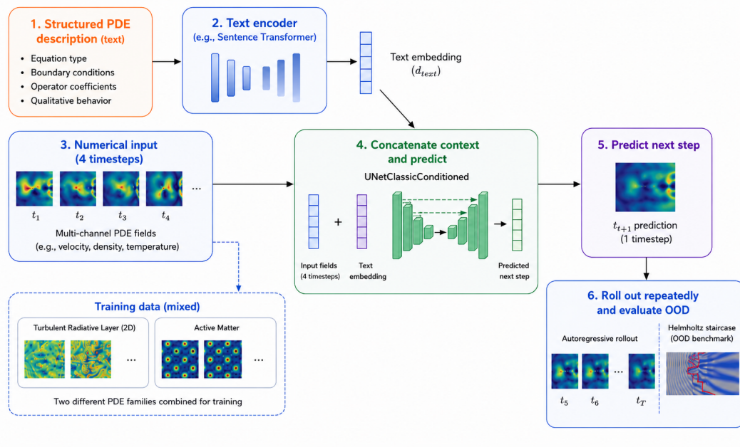
Figure 3: Experimental pipeline used in this project. The model combines structured PDE descriptions with numerical field histories, predicts the next timestep, and is evaluated through OOD rollout.
