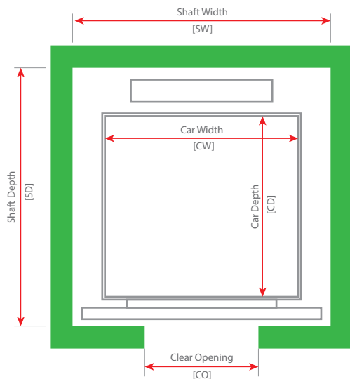
TYPICAL SHAFT AND CAR SIZE (AUTO DOOR PASSENGER LIFT)
