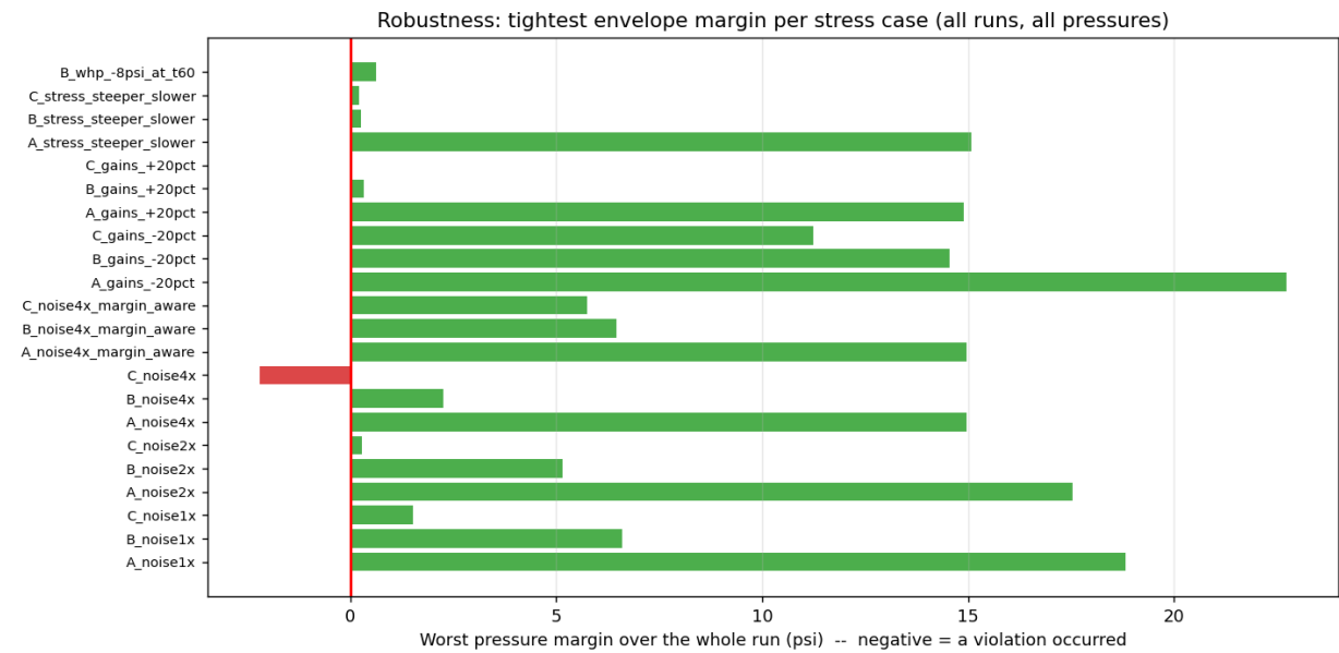
Figure 7 - Robustness: tightest envelope margin across 22 stress cases
