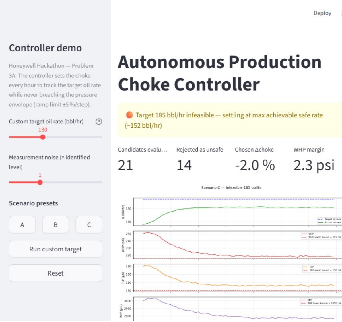
Figure 9 - Live dashboard (streamlit run app.py): Scenario C mid-refusal - 14 of 21 candidate moves rejected as unsafe, 2.3 psi WHP margin
