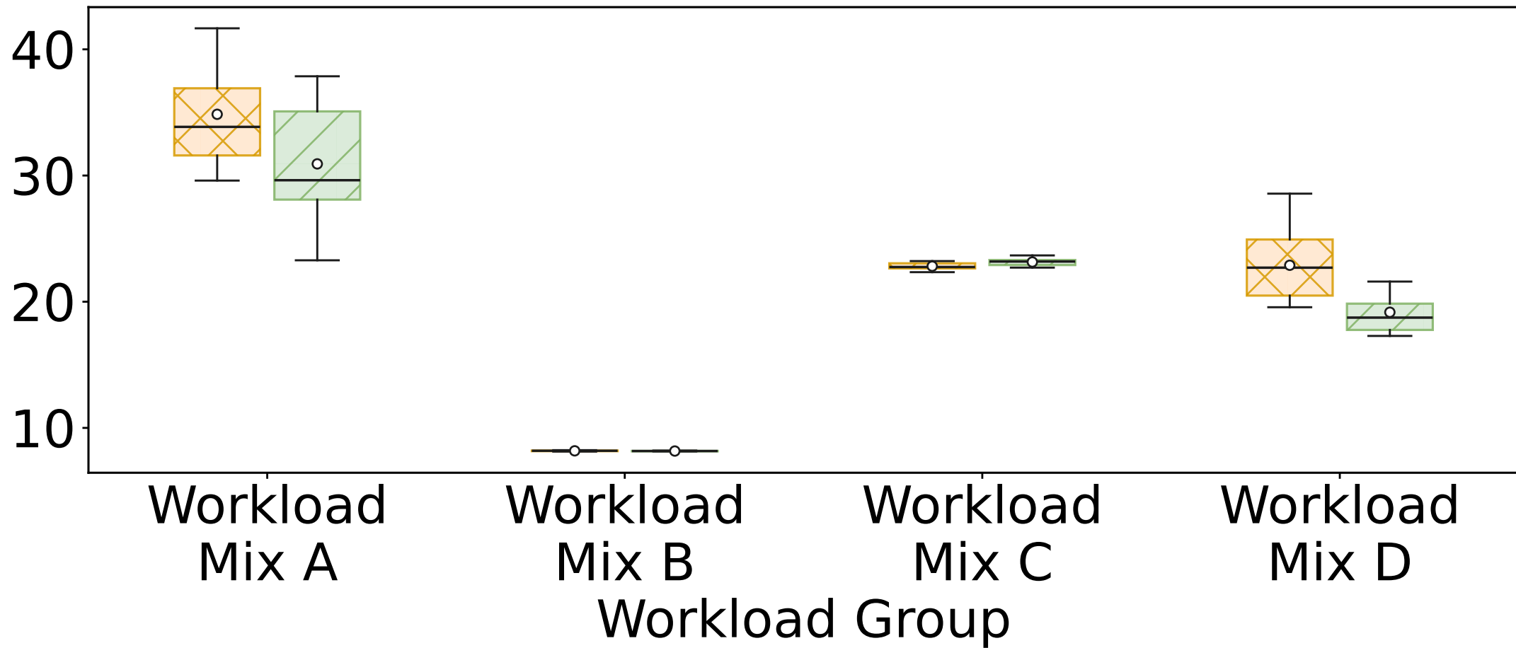
Per-Run Mean Core Utilization Imbalance (%)
