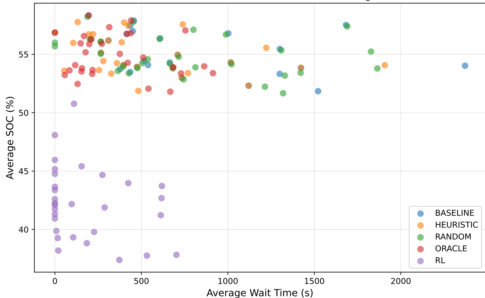
Wait Time vs SOC Trade-off Across Strategies
