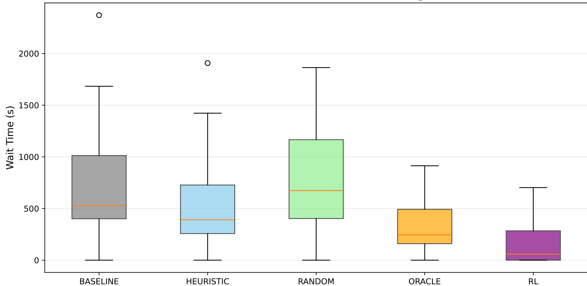
Distribution of Wait Times Across Strategies
