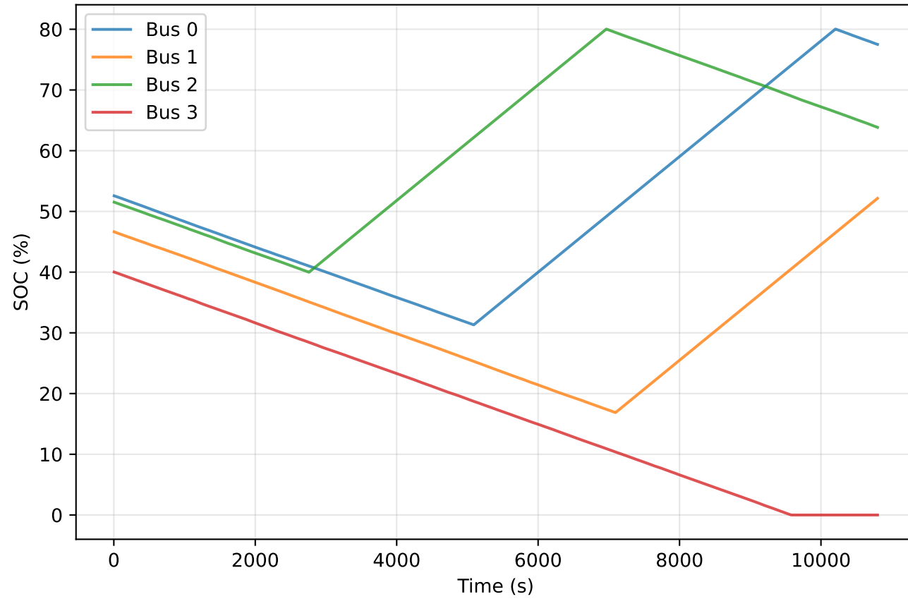
Charging Queue Dynamics
