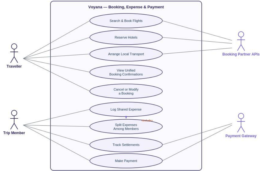
Figure 2. Use case diagram - booking, expense and payment.
