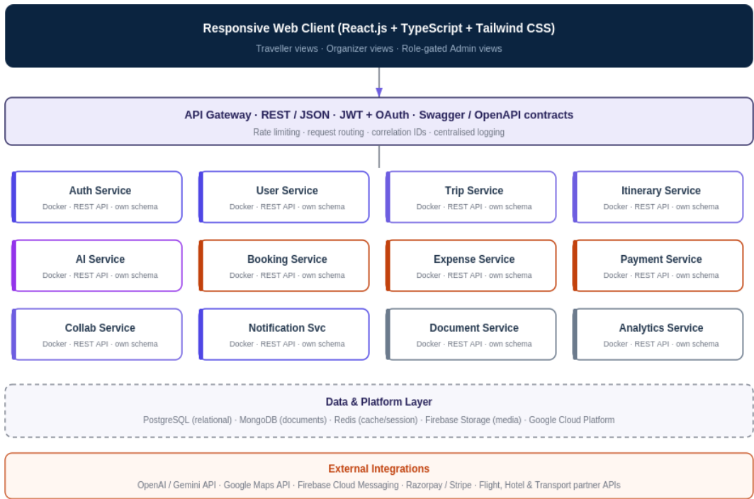
Figure 5. Voyana system context and service decomposition.
