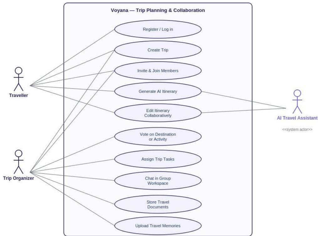
Figure 1. Use case diagram - trip planning and collaboration.
