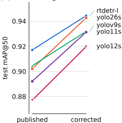
(a) test mAP@50
