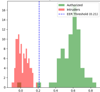
Similarity Distribution
