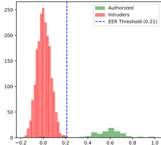
Similarity Distribution
