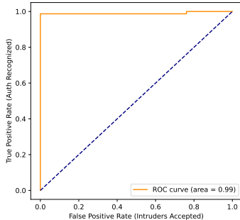
ROC Curve
