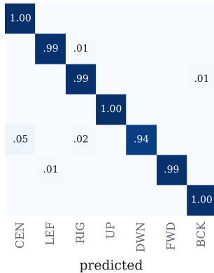
(b) session B acc 0.988
