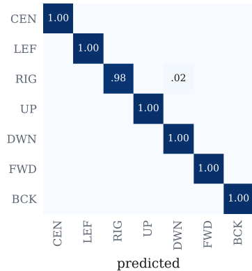
(a) session A acc 0.997
