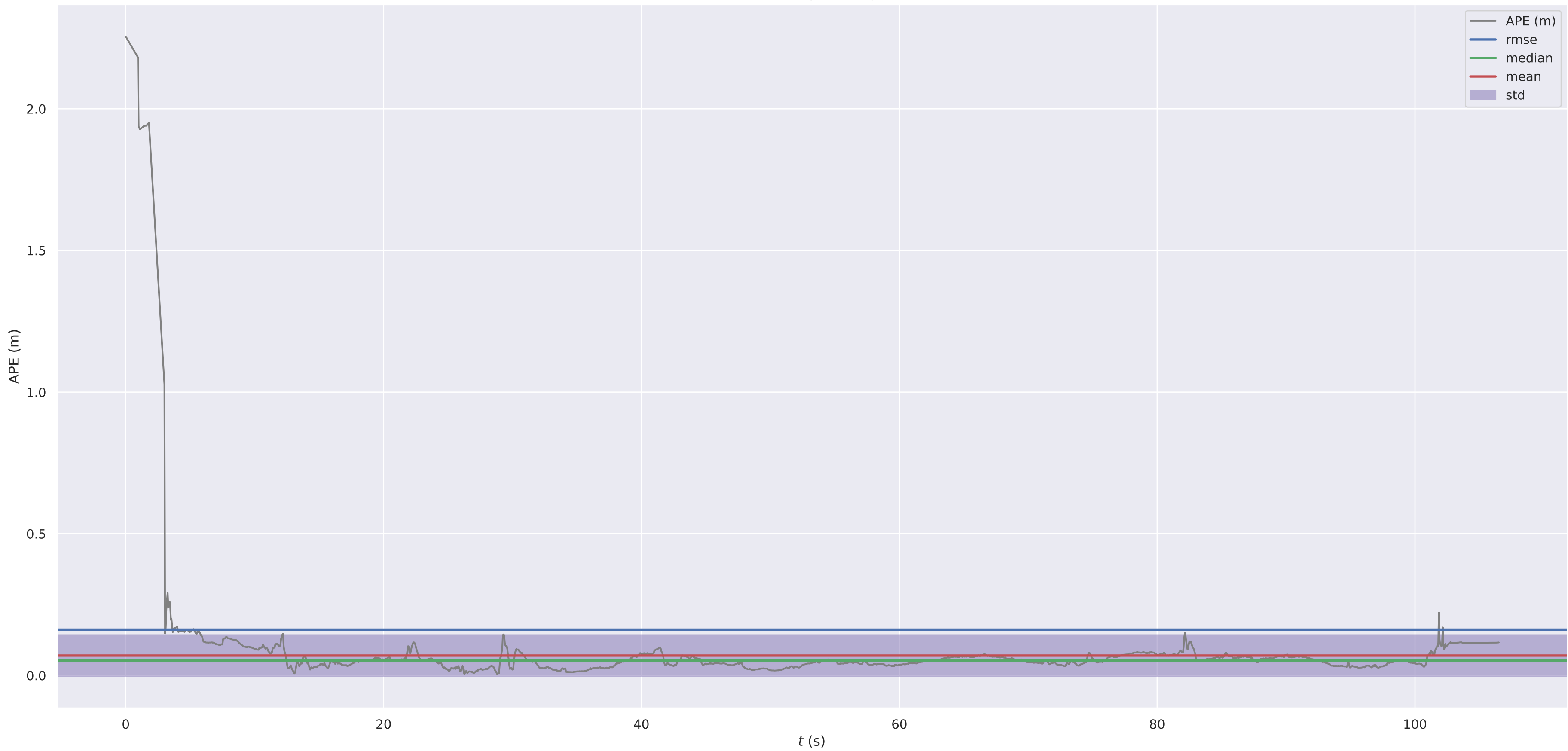
APE w.r.t. translation part (m) (with SE(3) Umeyama alignment)
