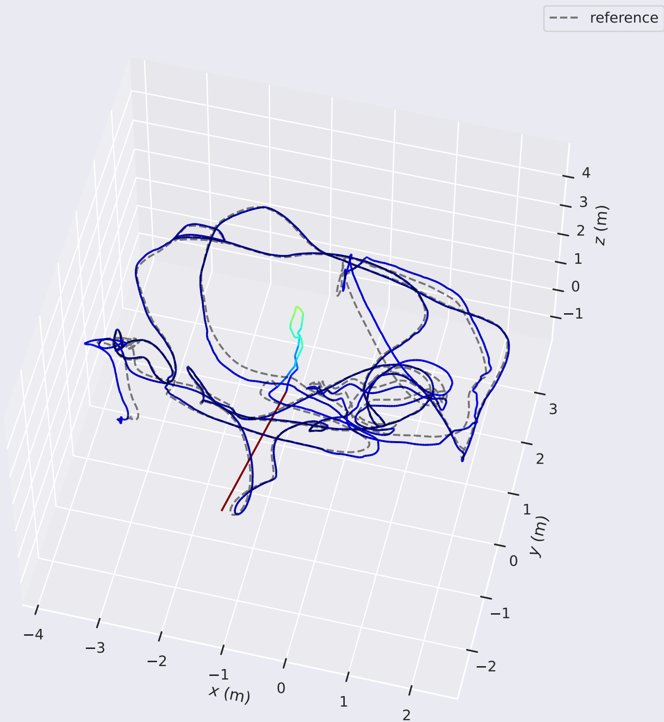
APE w.r.t. translation part (m) (with SE(3) Umeyama alignment)
