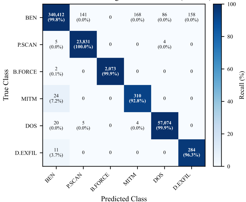
Confusion Matrix — LightGBM Classifier (Test Set)
