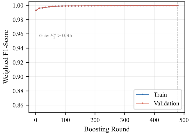
(b) Training and Validation F1-Score
