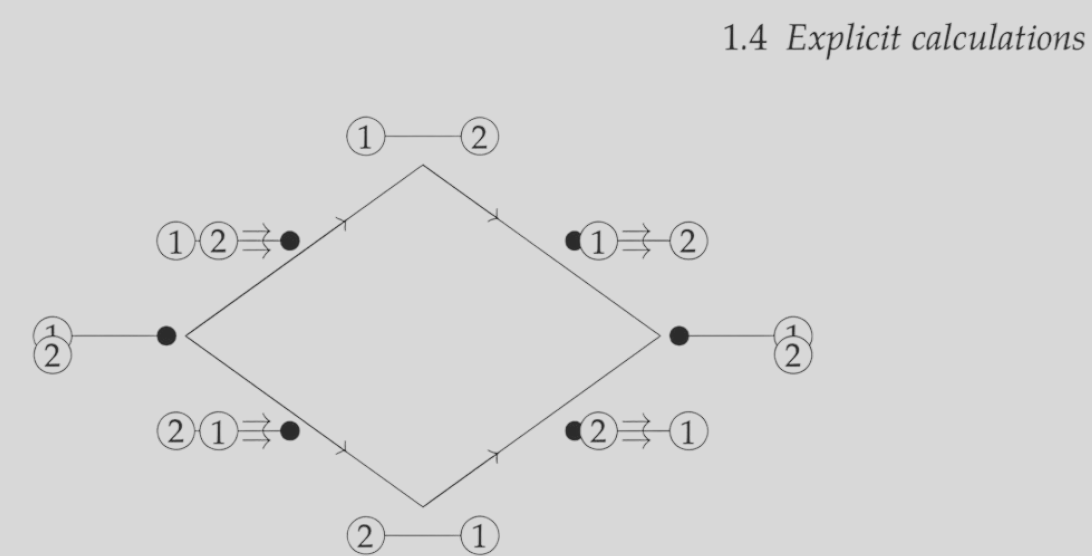
Figure 1.4: The combinatorial model of \text{Conf}_2(I, \{0, 1\}) consists of four edges.
