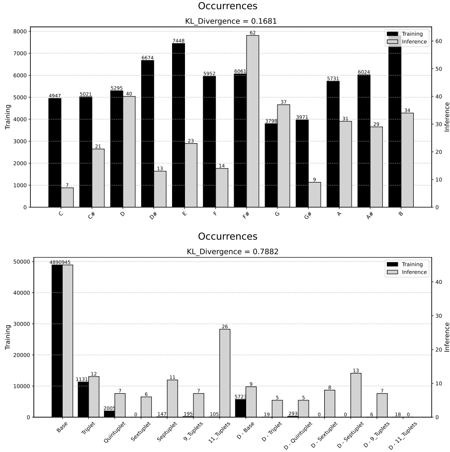
Figure 5: Note and beat occurrences of training data and inference
