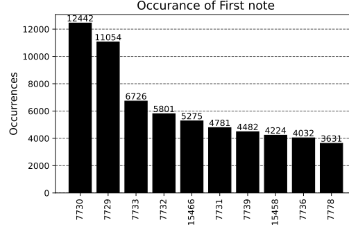
Figure 4: Distribution of starting notes for musical measures, used to select initial tokens at inference time for more consistent generation.
