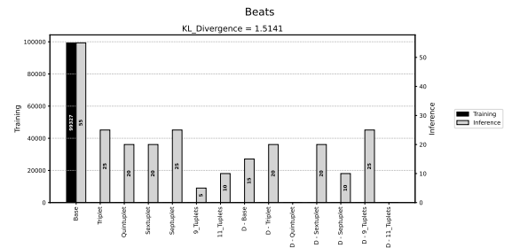
Figure 7: KL divergence for beat tokens with start token 15528, showing the model preserves rhythmic structure.
