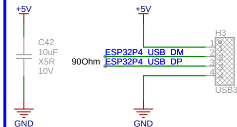
ESP32-P4 USB Host
