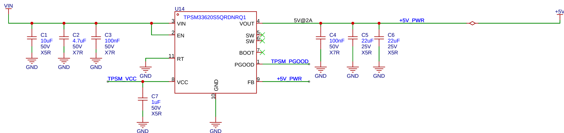
High Input Voltage Buck Converter
