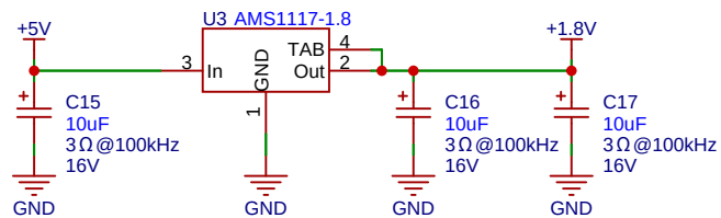
1.8V LDO
