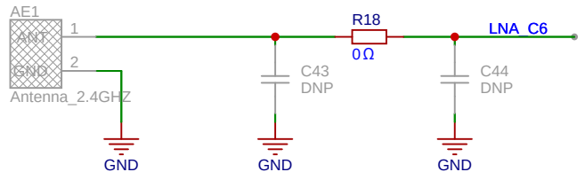
2.4GHz PCB Antenna
