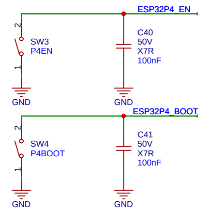
Strapping & Boot
