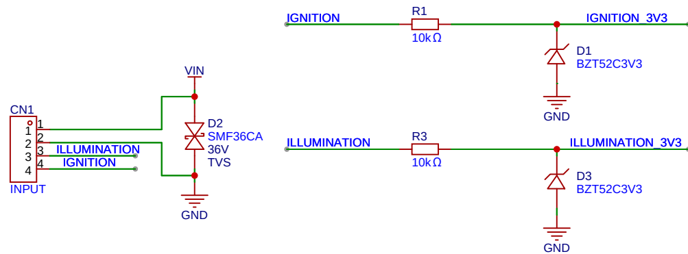
12V - 36V Input With Protection
