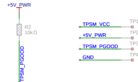
Pull-ups & Test Points
