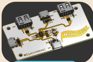
CUSTOM PCB
