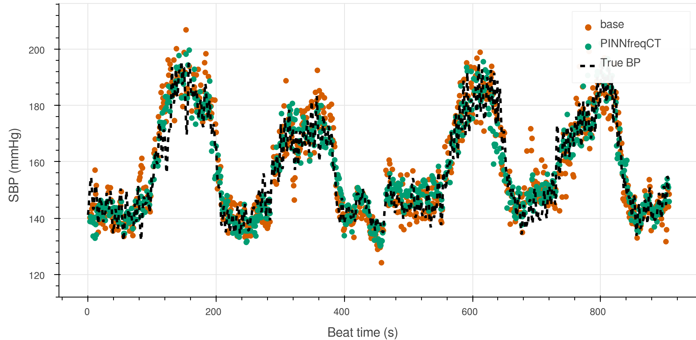
Robustness Test (Noise Level = 0.1)
