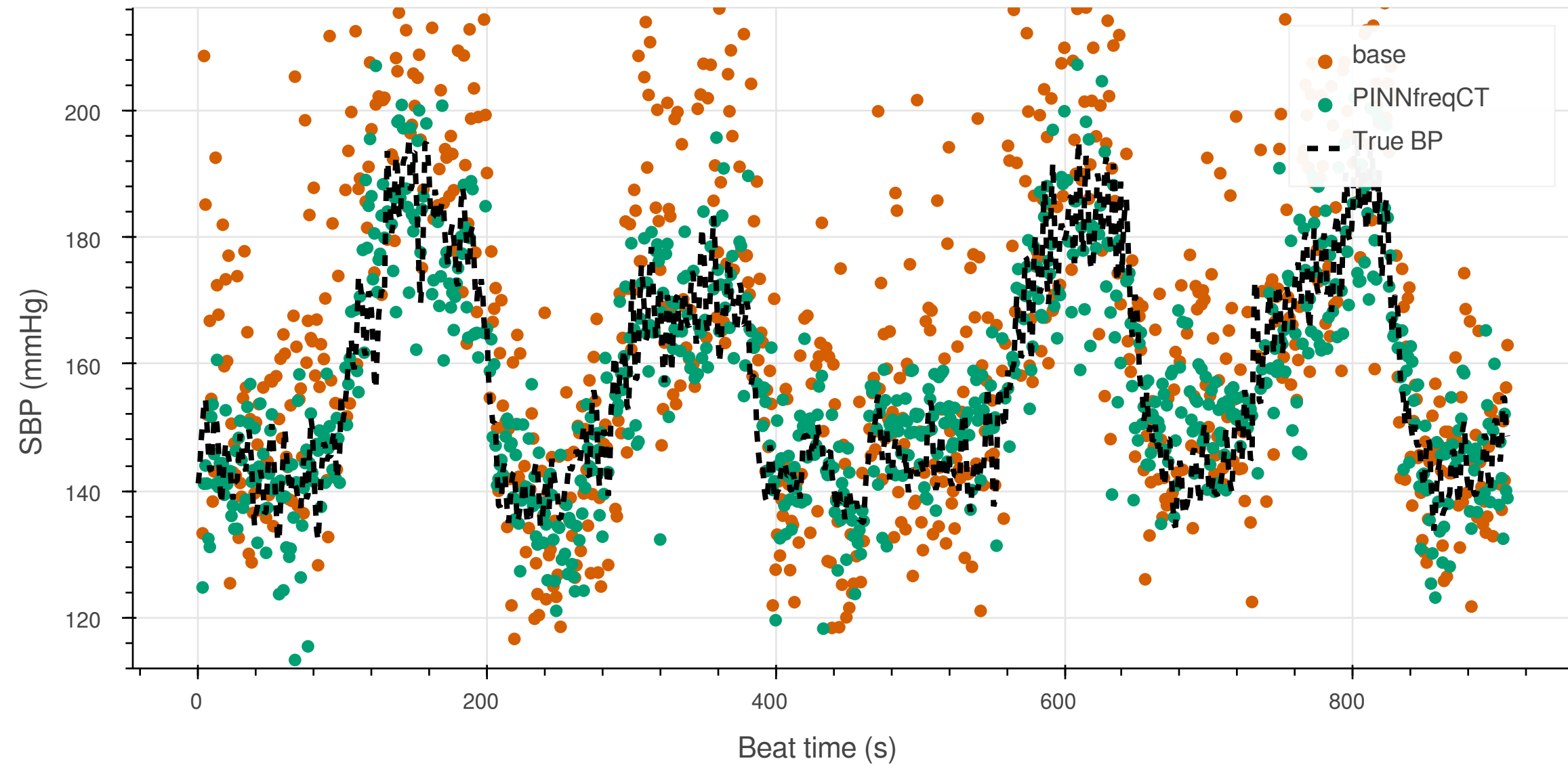
Robustness Test (Noise Level = 0.4)
