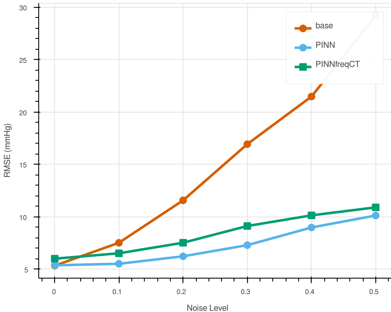
RMSE vs Noise (Lower is Better)
